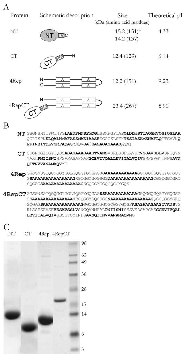
FIGURE 1: Description of the analyzed constructs. (A) Characteristics of recombinant E. australis MaSp1 proteins. White boxes represent polyaniline stretches, and black lines represent glycine rich regions. Gray boxes represent regions rich in serine and alanine. (B) Predictions of the secondary structures of the different parts. Segments predicted to be in \alpha -helical conformations are shown in bold. Only segments with at least four consecutive residues in an \alpha -helix conformation are shown. For NT, the segment in parentheses is present only in the NT* construct. (C) SDS-PAGE of purified NT, CT, 4Rep, and 4RepCT, as labeled above the lanes. Migration of low-molecular mass markers (kilodaltons) is shown at the right.
